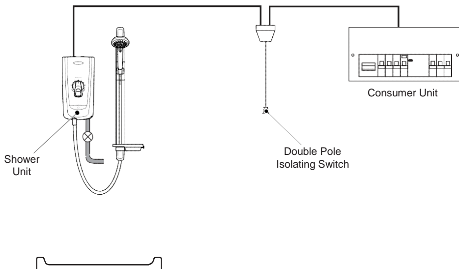
Electrical Schematic Diagram
